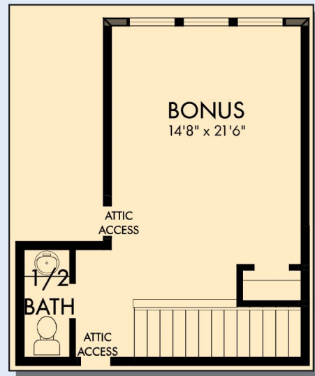
OPTIONAL THIRD FLOOR BONUS WITH HALF BATH
