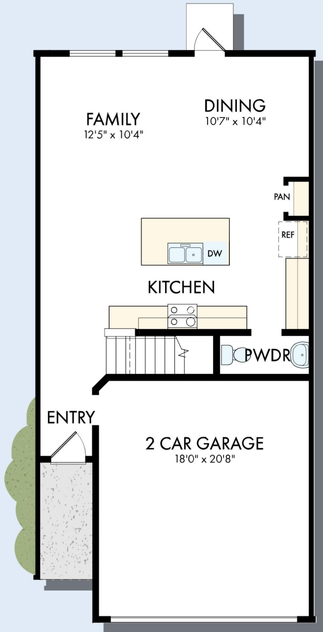
FIRST FLOOR
