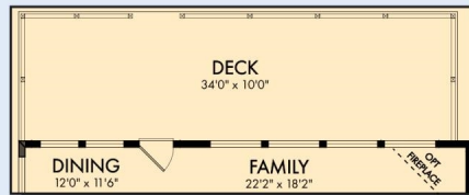
OPTIONAL EXTENDED DECK AT FAMILY AND DINING
