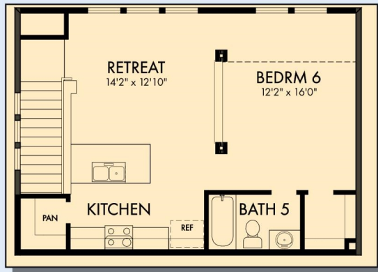
OPTIONAL SECOND FLOOR GARAGE RETREAT ABOVE 2 CAR GARAGE
