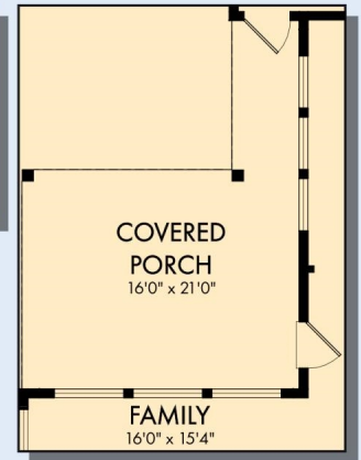
OPTIONAL EXTENDED COVERED PORCH
