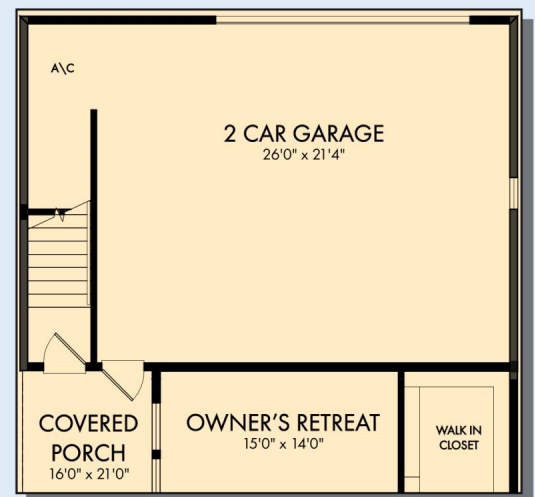
FIRST FLOOR WITH OPTIONAL RETREAT ABOVE 2 CAR GARAGE
