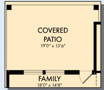
OPTIONAL EXTENDED COVERED PATIO
