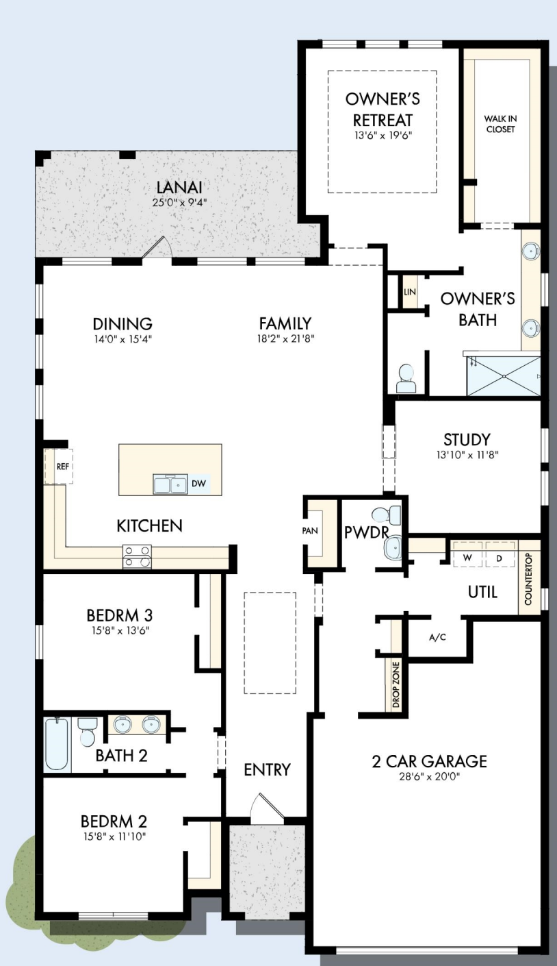
OPTIONAL EXTENDED LANAI WITH SLIDING GLASS DOOR
