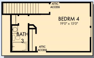
OPTIONAL SECOND FLOOR BEDROOM 4 AND BATH 3
