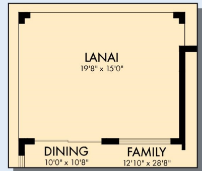
OPTIONAL EXTENDED LANAI WITH SLIDING GLASS DOOR AT DINING
