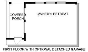
FIRST FLOOR WITH OPTIONAL DETACHED GARAGE
