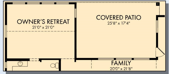
OPTIONAL EXTENDED COVERED PATIO WITH EXTENDED OWNER'S RETREAT
