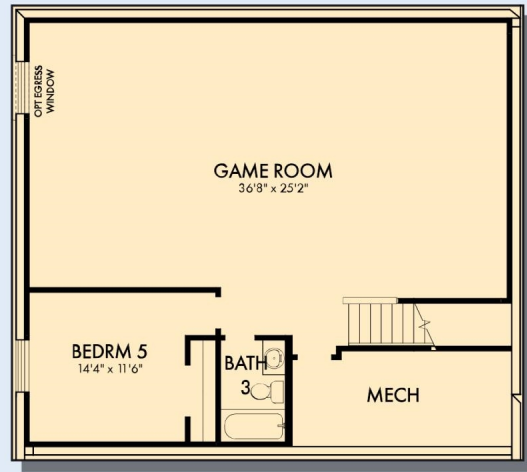
OPTIONAL GAME ROOM WITH BEDRM 5 AND BATH 3 AT BASEMENT
