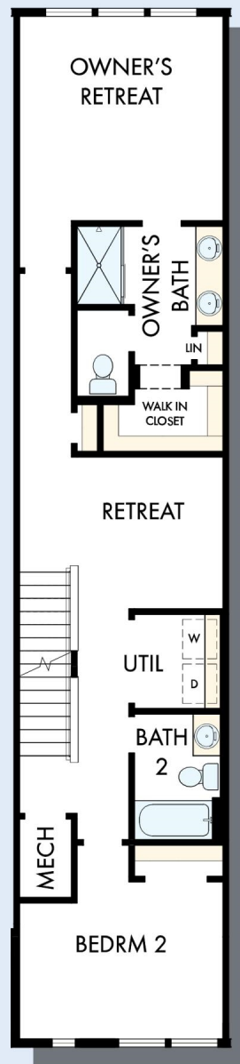
SECOND FLOOR
