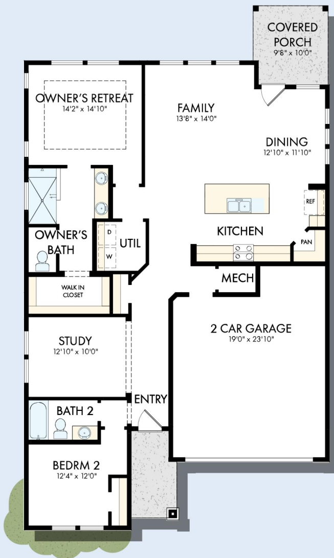
OPTIONAL EXTENDED COVERED PORCH
