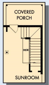
FIRST FLOOR WITH OPTIONAL BACK STAIRS
