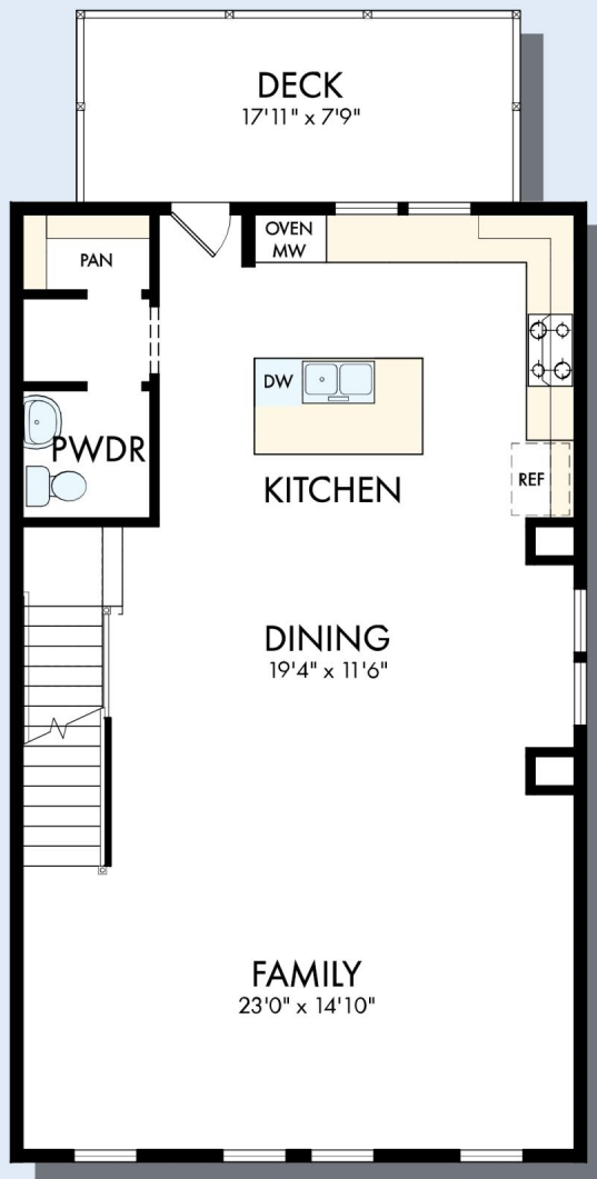
SECOND FLOOR
