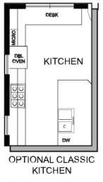
OPTIONAL CLASSIC KITCHEN
