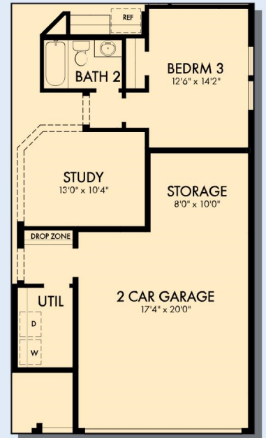
OPTIONAL STORAGE AT 2 CAR GARAGE
