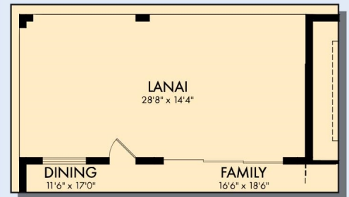
OPTIONAL EXTENDED LANAI WITH SLIDING GLASS DOOR
