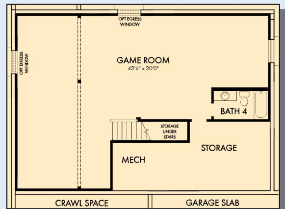
OPTIONAL GAME ROOM WITH BATH 4 AT BASEMENT
