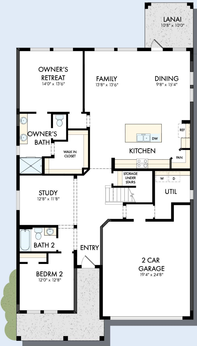
FIRST FLOOR
