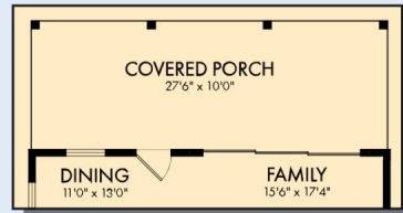
OPTIONAL EXTENDED COVERED PORCH WITH SLIDING GLASS DOOR
