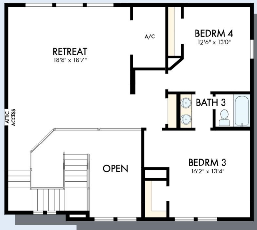
SECOND FLOOR
