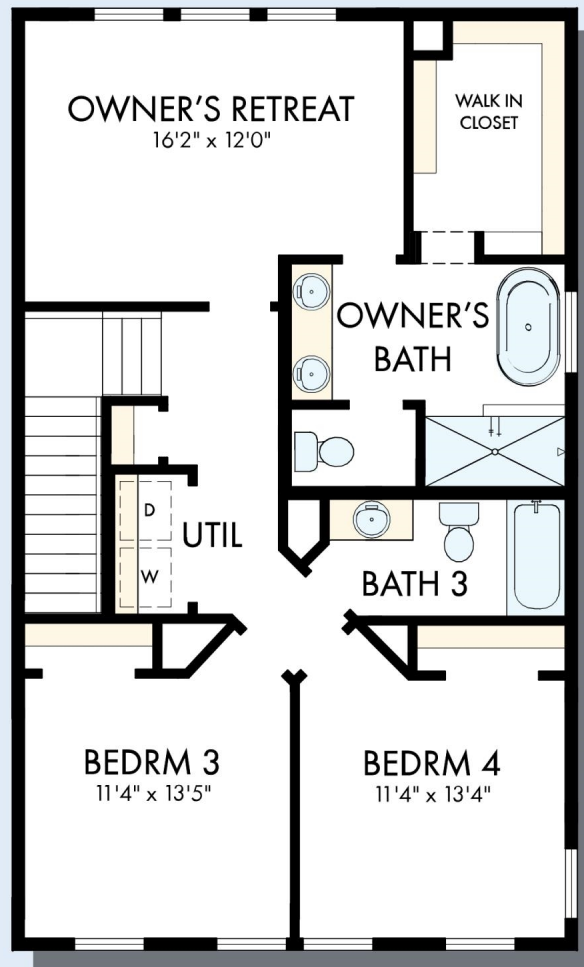
THIRD FLOOR
