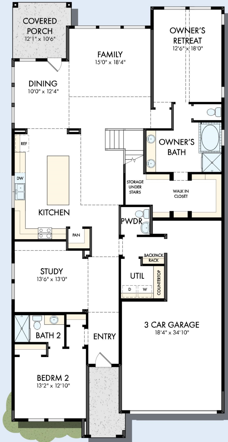
FIRST FLOOR
