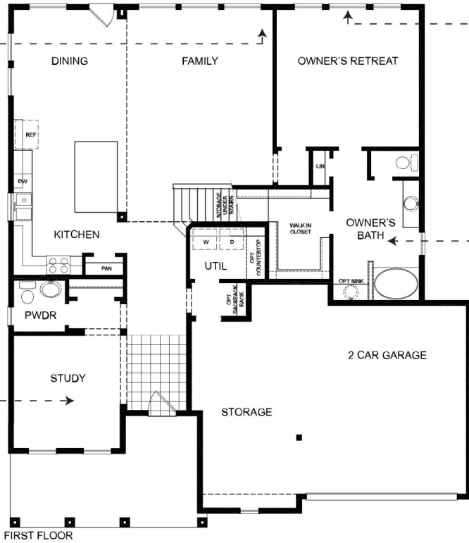
OPTIONAL ENCLOSED STUDY WITH FRENCH DOORS
