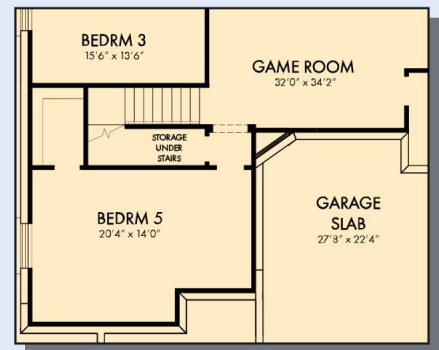
OPTIONAL BEDROOM 5 AT STORAGE
