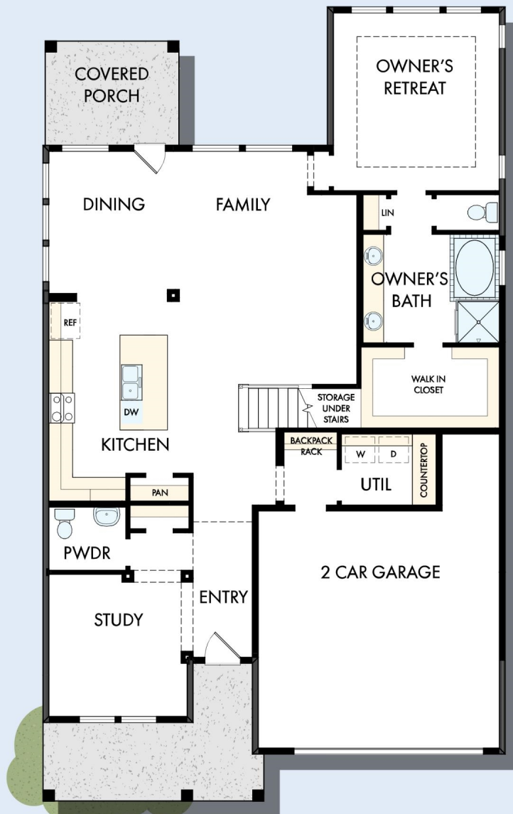
FIRST FLOOR
