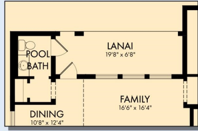
OPTIONAL POOL BATH AT LANAI
