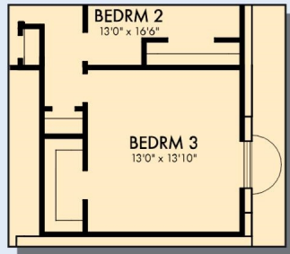
OPTIONAL BEDROOM 3 AT BASEMENT
