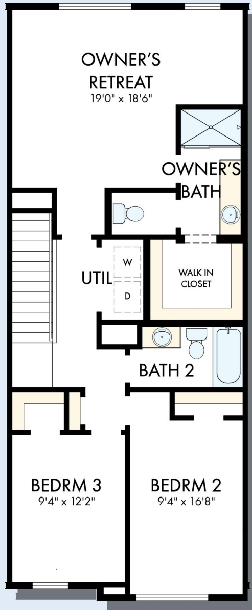
SECOND FLOOR
