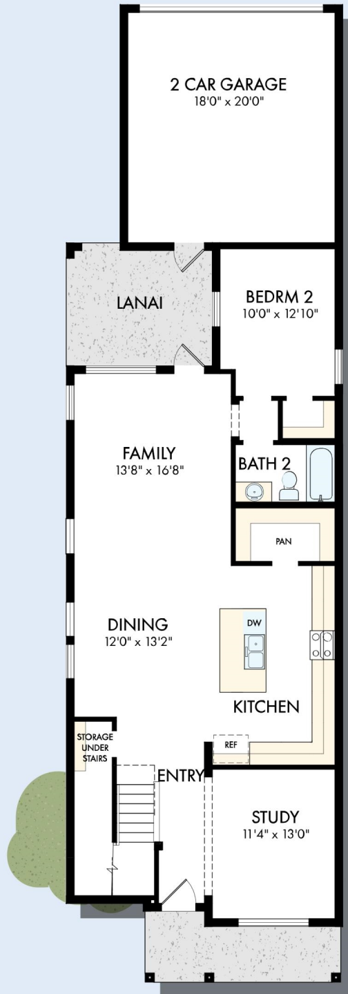
FIRST FLOOR
